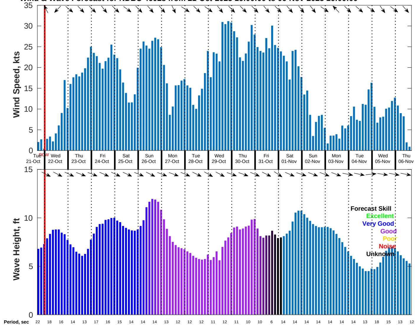
Wind & Wave Forecast for NDBC 46028 from 21-Oct-2025 16:00:00 to 06-Nov-2025 16:00:00
