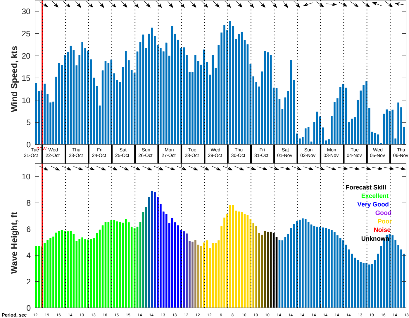
Wind & Wave Forecast for NDBC 46054 from 21-Oct-2025 16:00:00 to 06-Nov-2025 16:00:00
