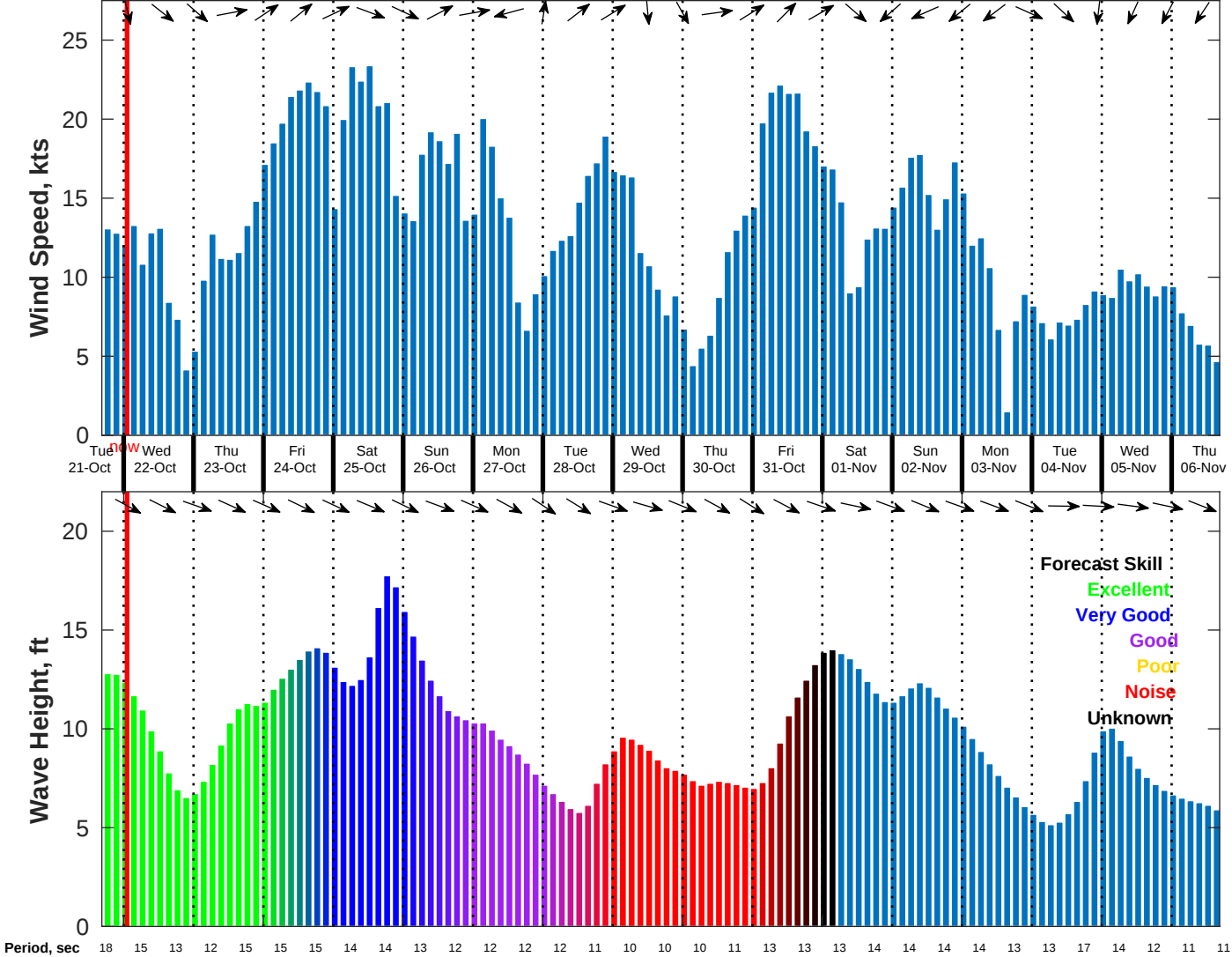
Wind & Wave Forecast for NDBC 46059 from 21-Oct-2025 17:00:00 to 06-Nov-2025 17:00:00
