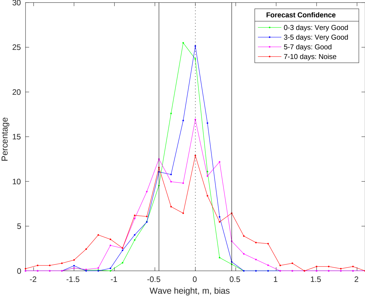
NDBC 46069 vs CMEMS Waves Bias Histogram: 22-Oct-2025
