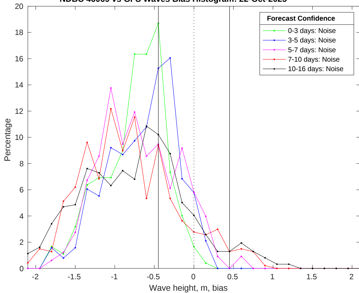
NDBC 46069 vs GFS Waves Bias Histogram: 22-Oct-2025
