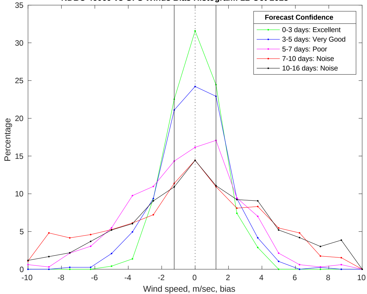
NDBC 46069 vs GFS Winds Bias Histogram: 22-Oct-2025
