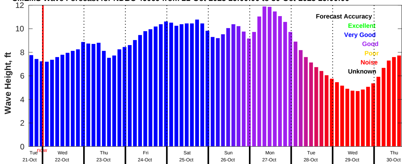
CMEMS Wave Forecast for NDBC 46069 from 21-Oct-2025 16:00:00 to 30-Oct-2025 16:00:00
