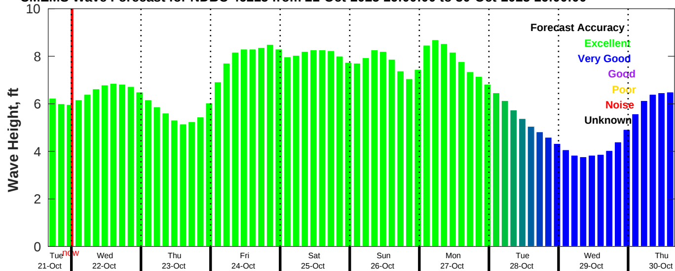
CMEMS Wave Forecast for NDBC 46215 from 21-Oct-2025 16:00:00 to 30-Oct-2025 16:00:00
