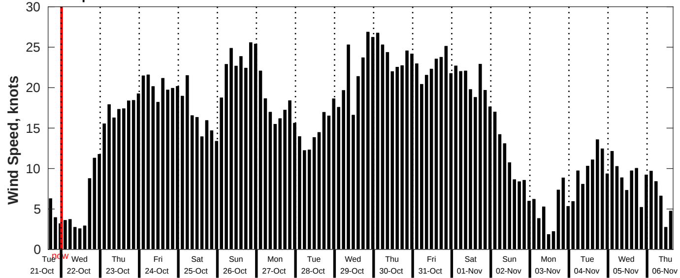
GFS Wind Speed Forecast for NDBC 46259 from 21-Oct-2025 16:00:00 to 06-Nov-2025 16:00:00
