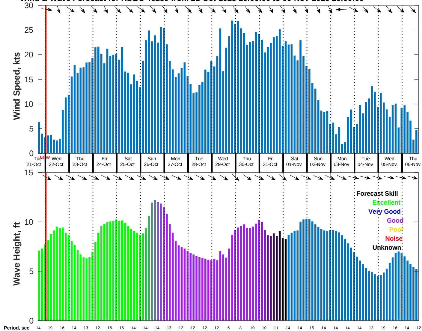
Wind & Wave Forecast for NDBC 46259 from 21-Oct-2025 16:00:00 to 06-Nov-2025 16:00:00
