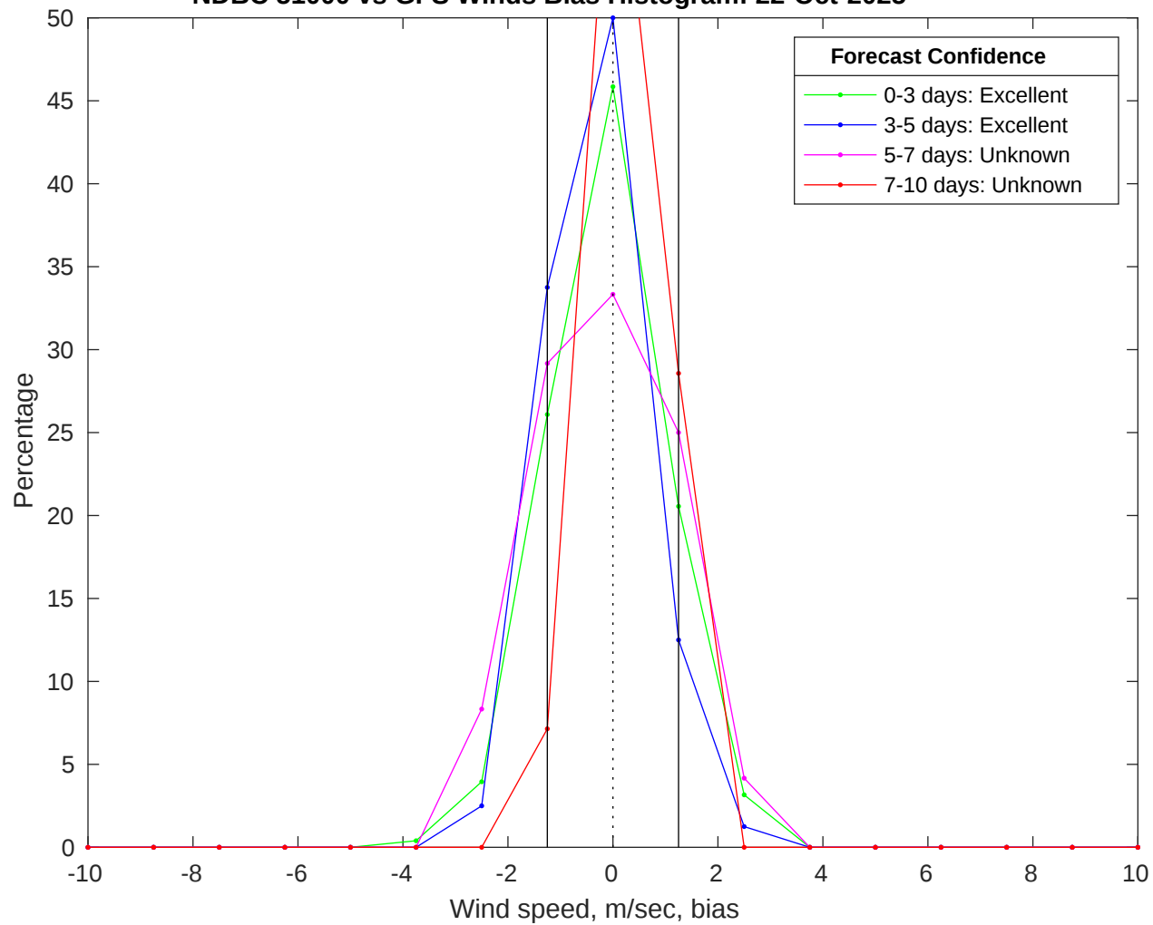
NDBC 51000 vs GFS Winds Bias Histogram: 22-Oct-2025
