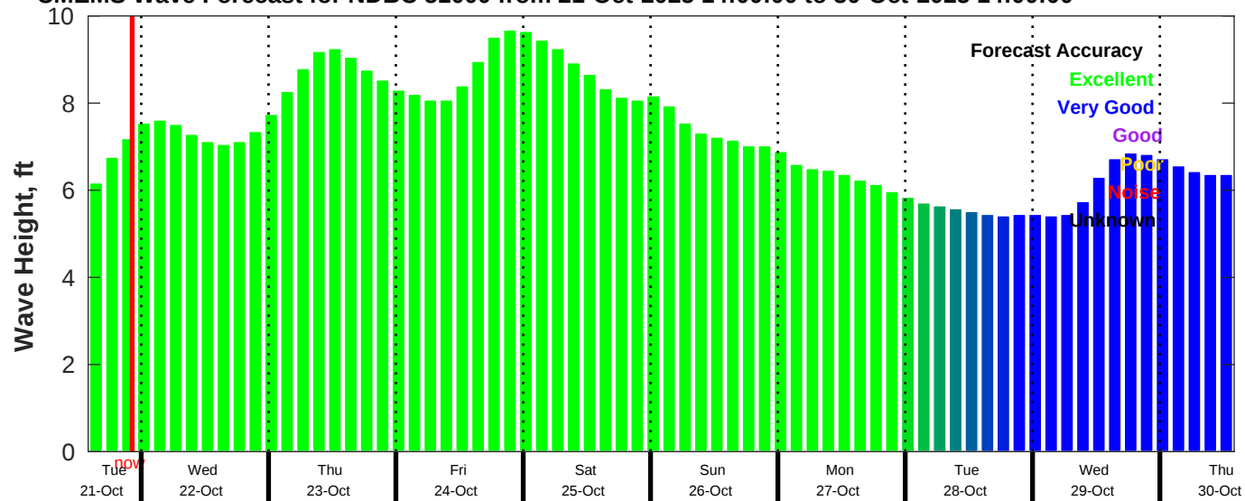
CMEMS Wave Forecast for NDBC 51000 from 21-Oct-2025 14:00:00 to 30-Oct-2025 14:00:00
