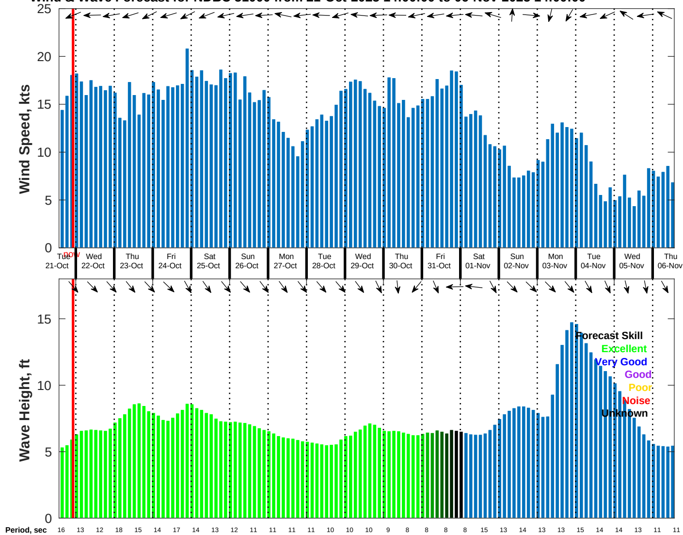
Wind & Wave Forecast for NDBC 51000 from 21-Oct-2025 14:00:00 to 06-Nov-2025 14:00:00
