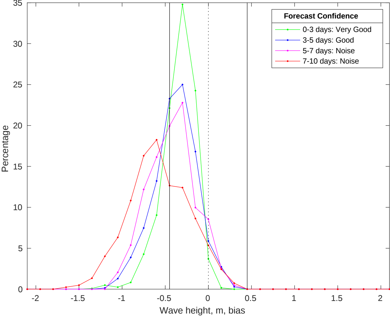
NDBC 51209 vs CMEMS Waves Bias Histogram: 22-Oct-2025
