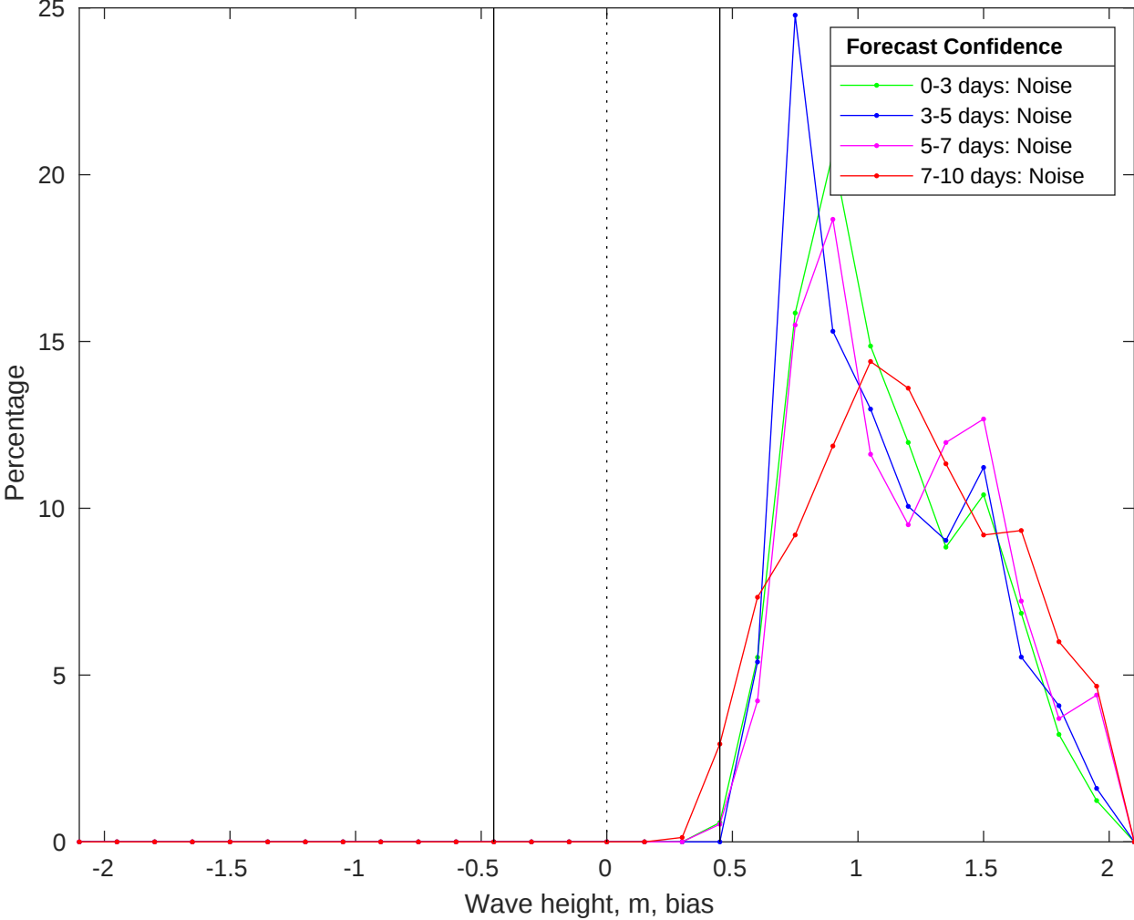
NDBC 51211 vs CMEMS Waves Bias Histogram: 22-Oct-2025
