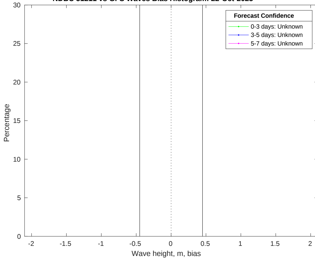
NDBC 51211 vs GFS Waves Bias Histogram: 22-Oct-2025
