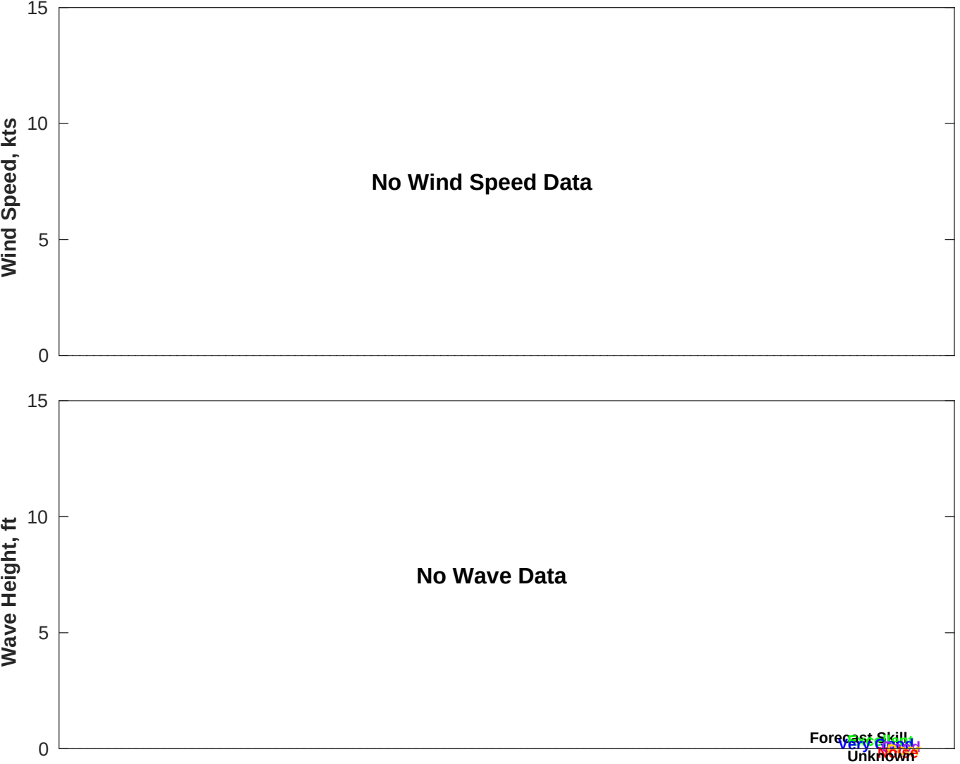
Wind & Wave Forecast for NDBC 51211 from 21-Oct-2025 14:00:00 to 06-Nov-2025 14:00:00
