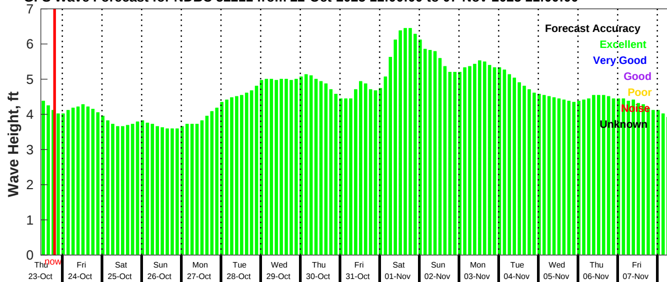
GFS Wave Forecast for NDBC 52211 from 22-Oct-2025 11:00:00 to 07-Nov-2025 11:00:00
