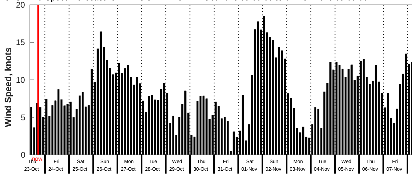
GFS Wind Speed Forecast for NDBC 52212 from 22-Oct-2025 09:00:00 to 07-Nov-2025 09:00:00
