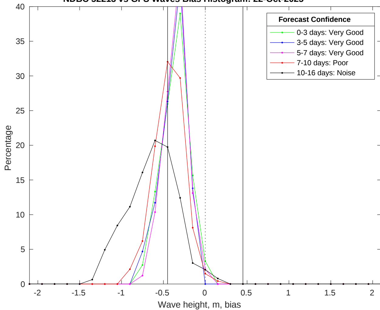
NDBC 52213 vs GFS Waves Bias Histogram: 22-Oct-2025
