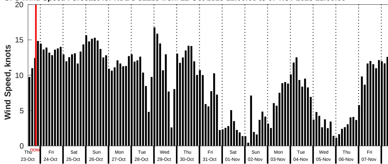
GFS Wind Speed Forecast for NDBC 52213 from 22-Oct-2025 11:00:00 to 07-Nov-2025 11:00:00
