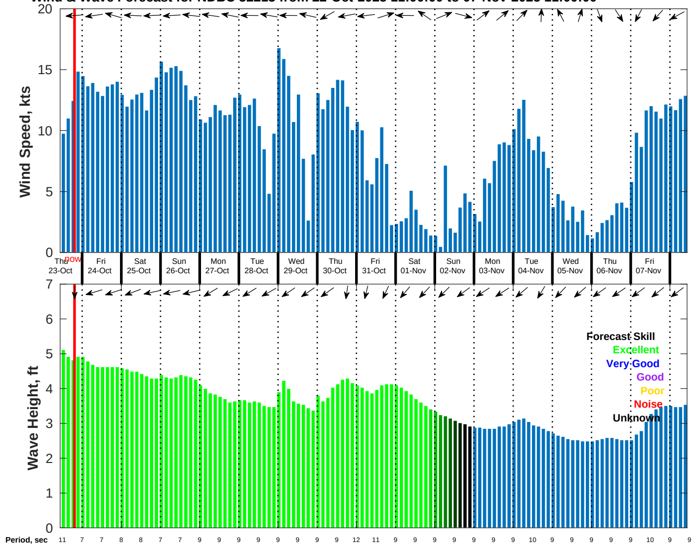
Wind & Wave Forecast for NDBC 52213 from 22-Oct-2025 11:00:00 to 07-Nov-2025 11:00:00
