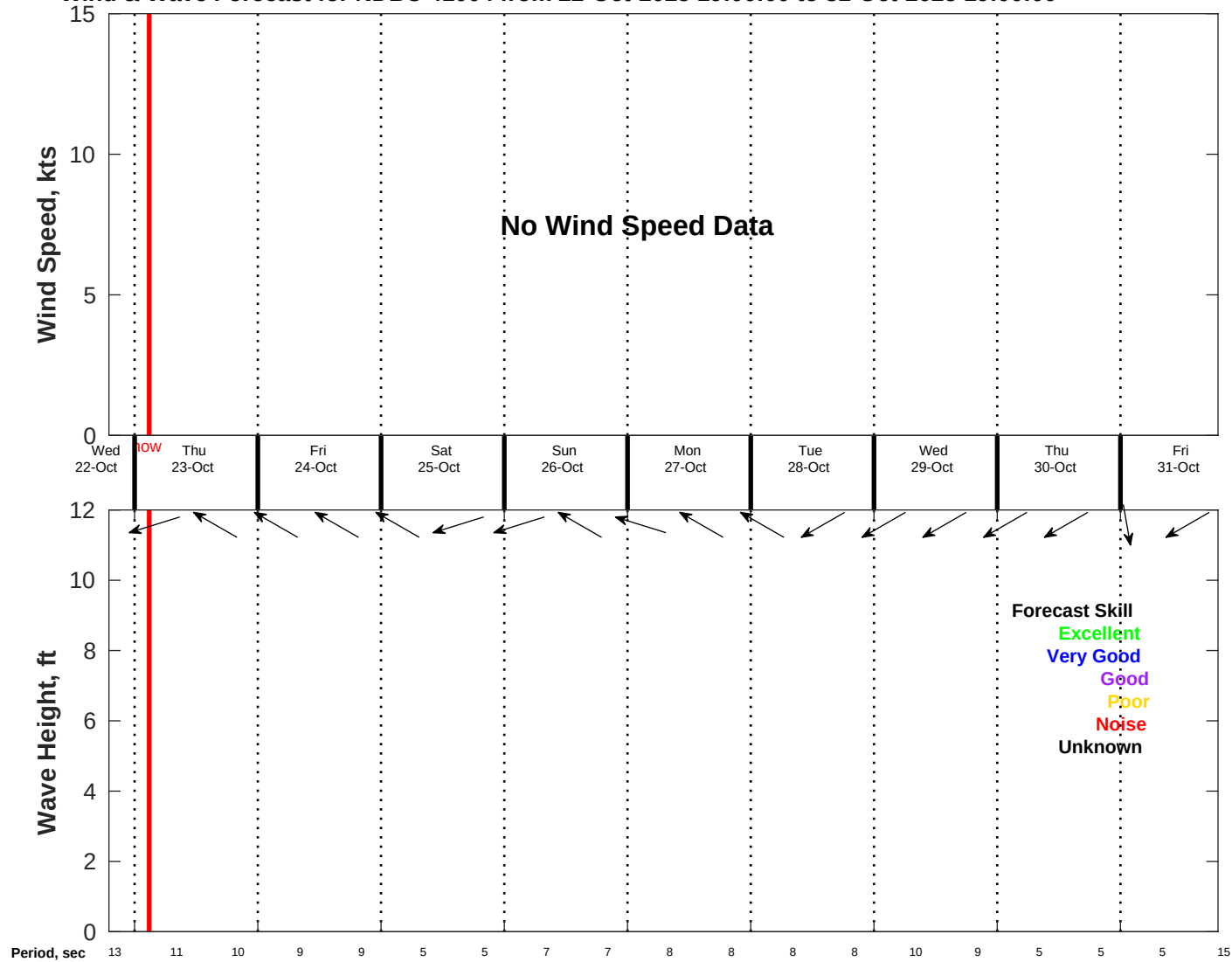
Wind & Wave Forecast for NDBC 41004 from 22-Oct-2025 19:00:00 to 31-Oct-2025 19:00:00
