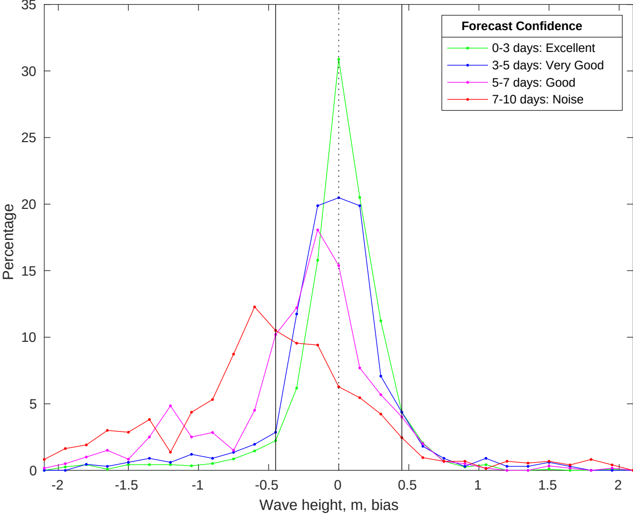
NDBC 41013 vs CMEMS Waves Bias Histogram: 23-Oct-2025
