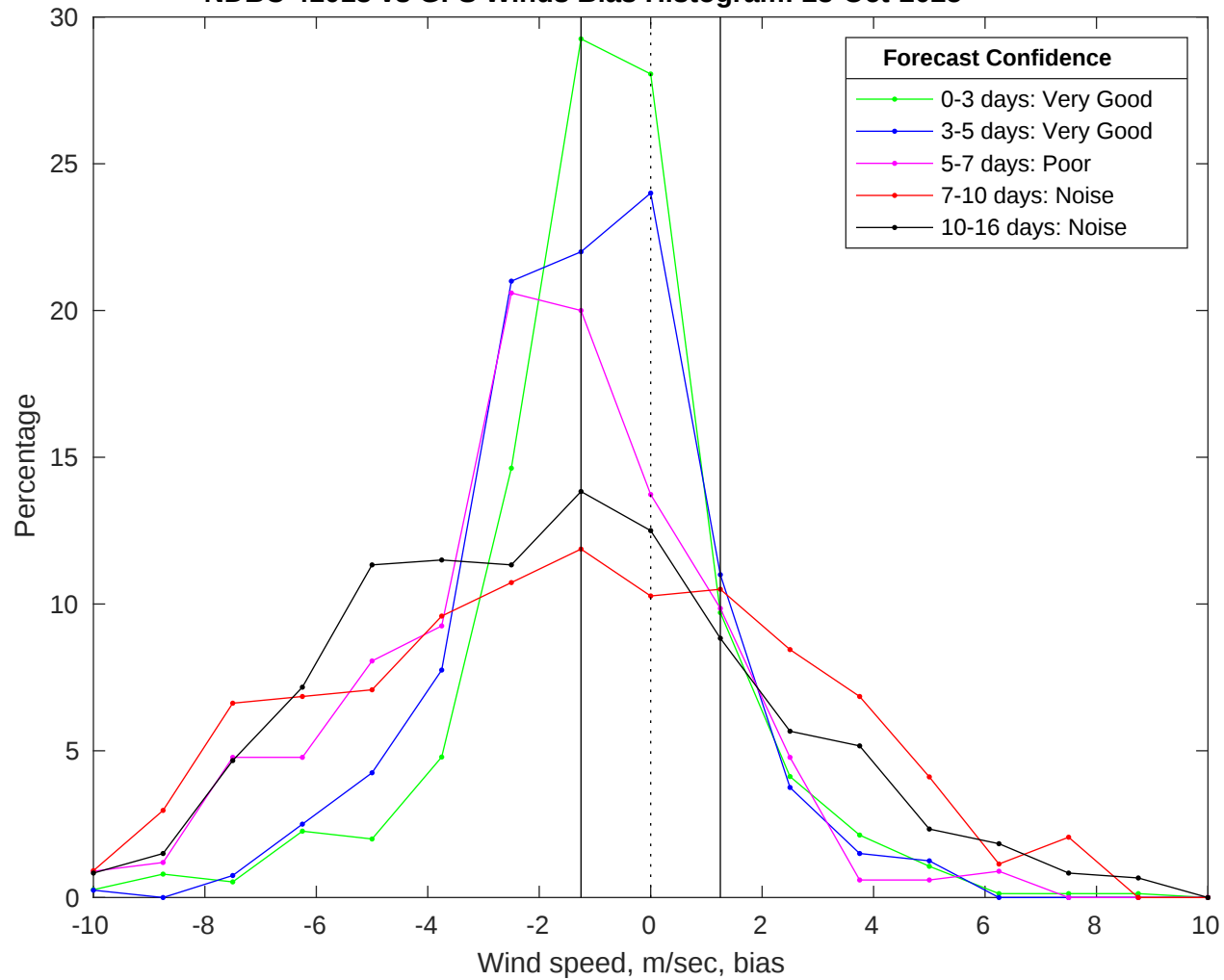
NDBC 41013 vs GFS Winds Bias Histogram: 23-Oct-2025
