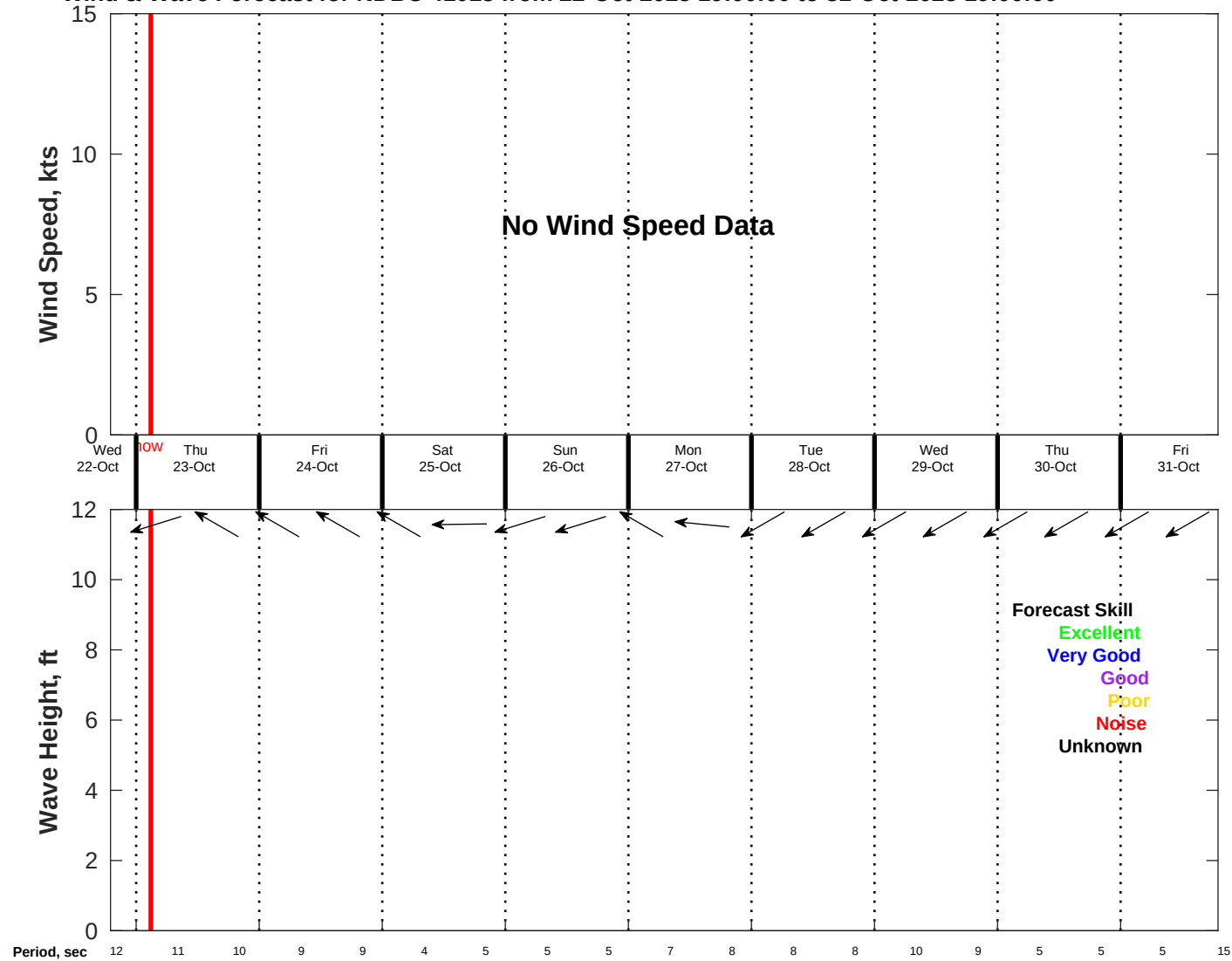
Wind & Wave Forecast for NDBC 41013 from 22-Oct-2025 19:00:00 to 31-Oct-2025 19:00:00
