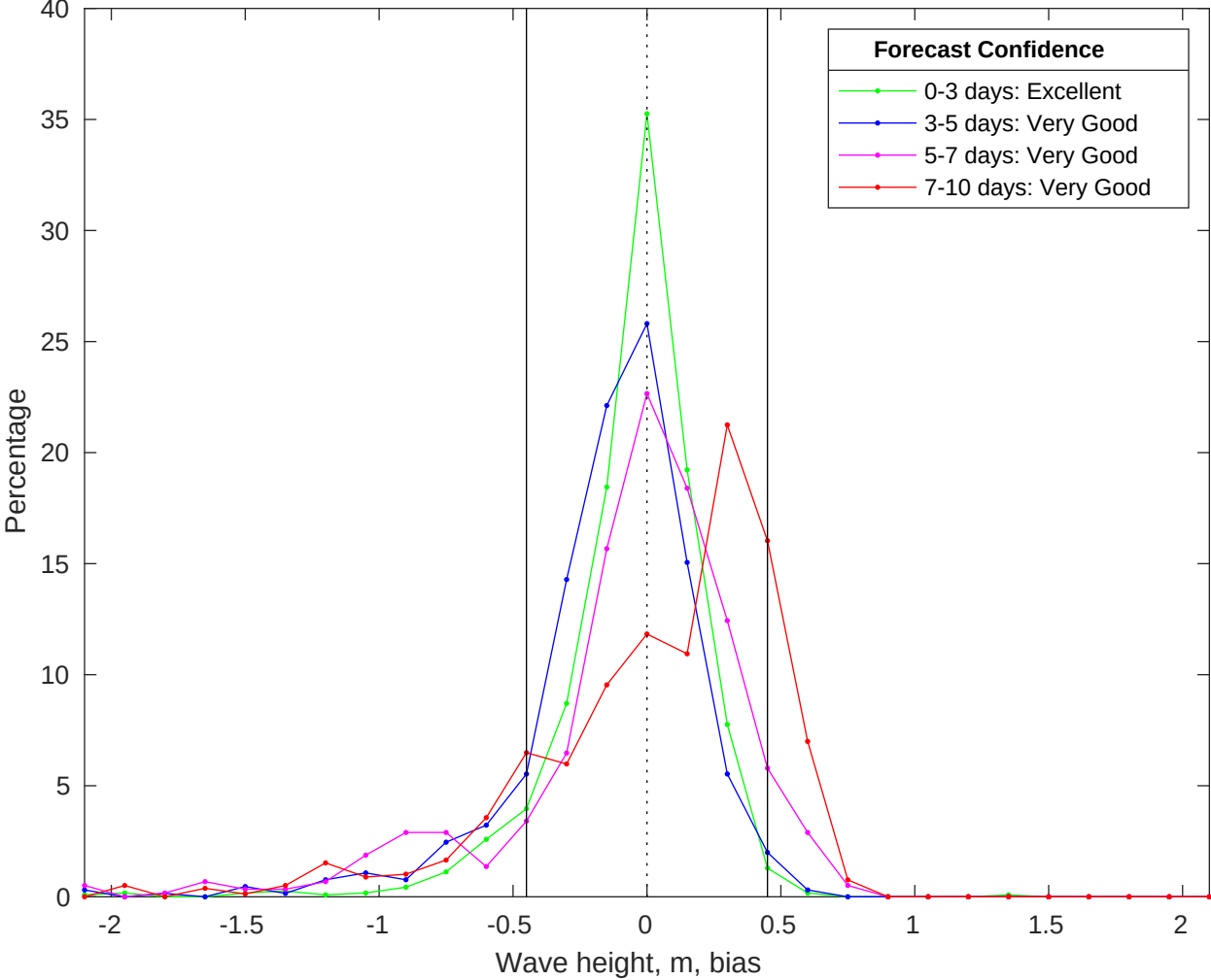
NDBC 41040 vs CMEMS Waves Bias Histogram: 23-Oct-2025
