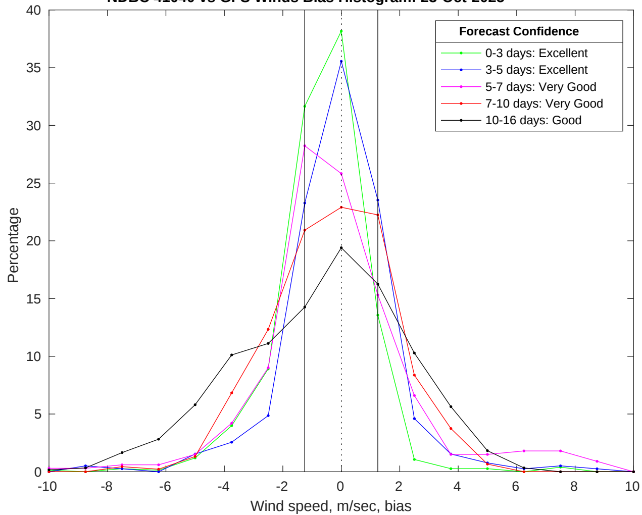
NDBC 41040 vs GFS Winds Bias Histogram: 23-Oct-2025
