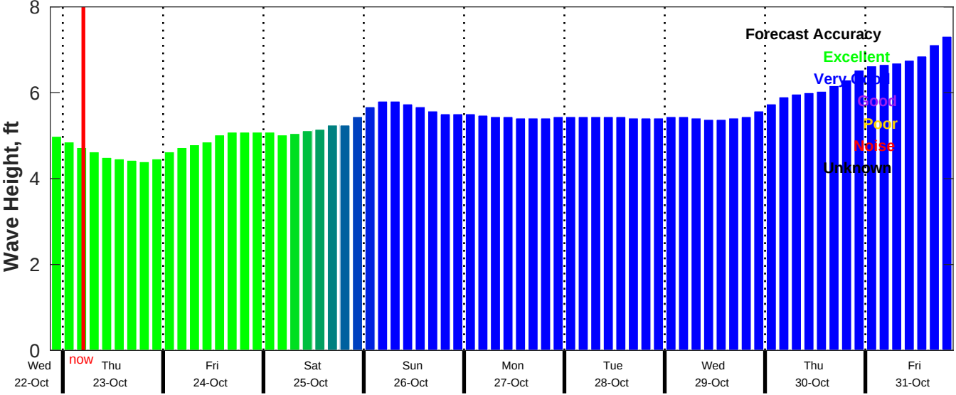
CMEMS Wave Forecast for NDBC 41040 from 22-Oct-2025 21:00:00 to 31-Oct-2025 21:00:00
