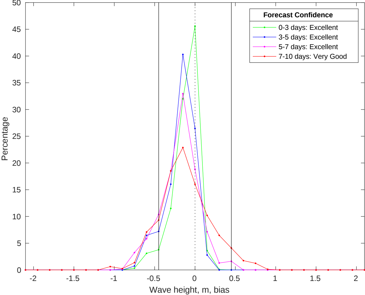
NDBC 42019 vs CMEMS Waves Bias Histogram: 23-Oct-2025
