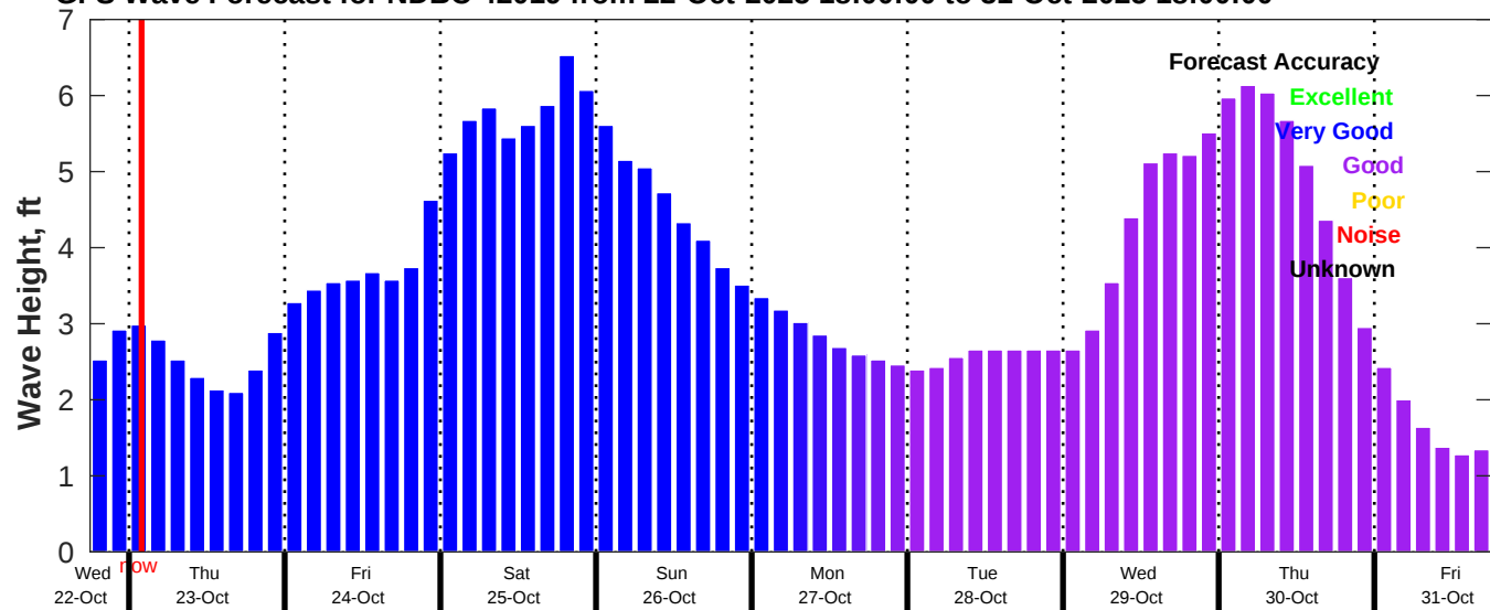
GFS Wave Forecast for NDBC 42019 from 22-Oct-2025 18:00:00 to 31-Oct-2025 18:00:00
