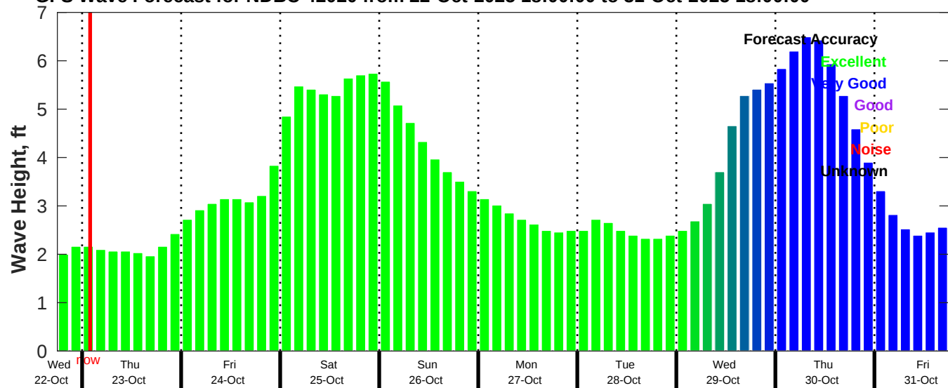
GFS Wave Forecast for NDBC 42020 from 22-Oct-2025 18:00:00 to 31-Oct-2025 18:00:00
