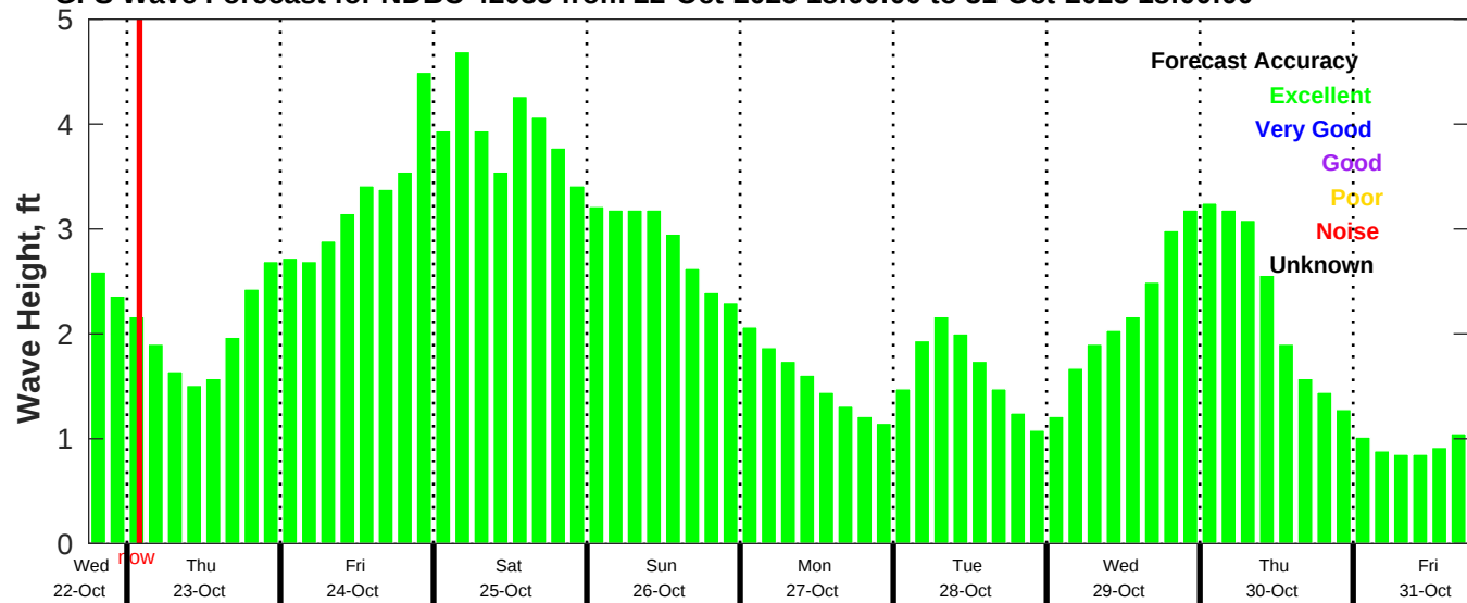
GFS Wave Forecast for NDBC 42035 from 22-Oct-2025 18:00:00 to 31-Oct-2025 18:00:00
