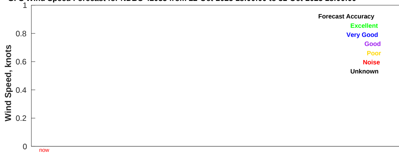
GFS Wind Speed Forecast for NDBC 42035 from 22-Oct-2025 18:00:00 to 31-Oct-2025 18:00:00
