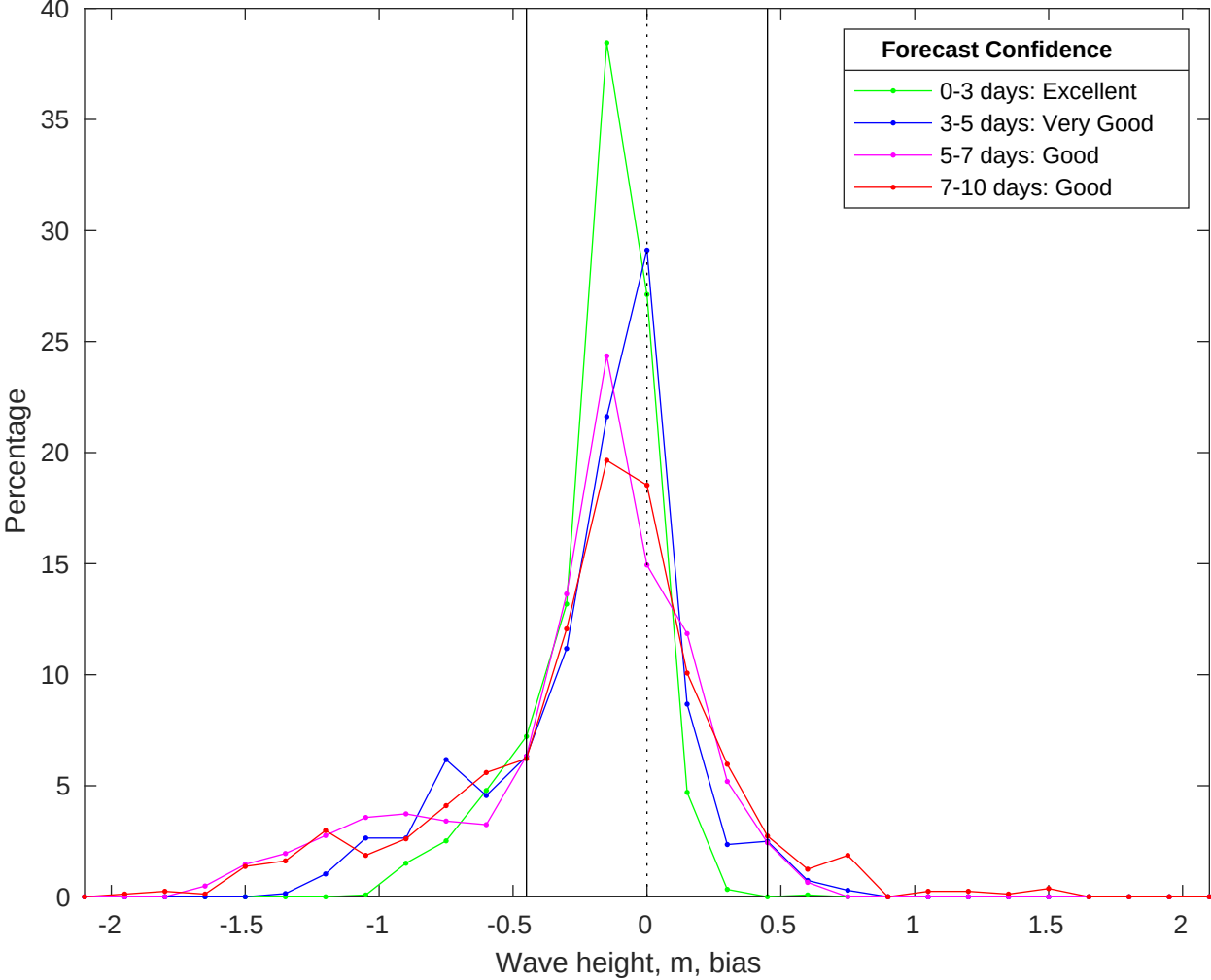
NDBC 42036 vs CMEMS Waves Bias Histogram: 23-Oct-2025
