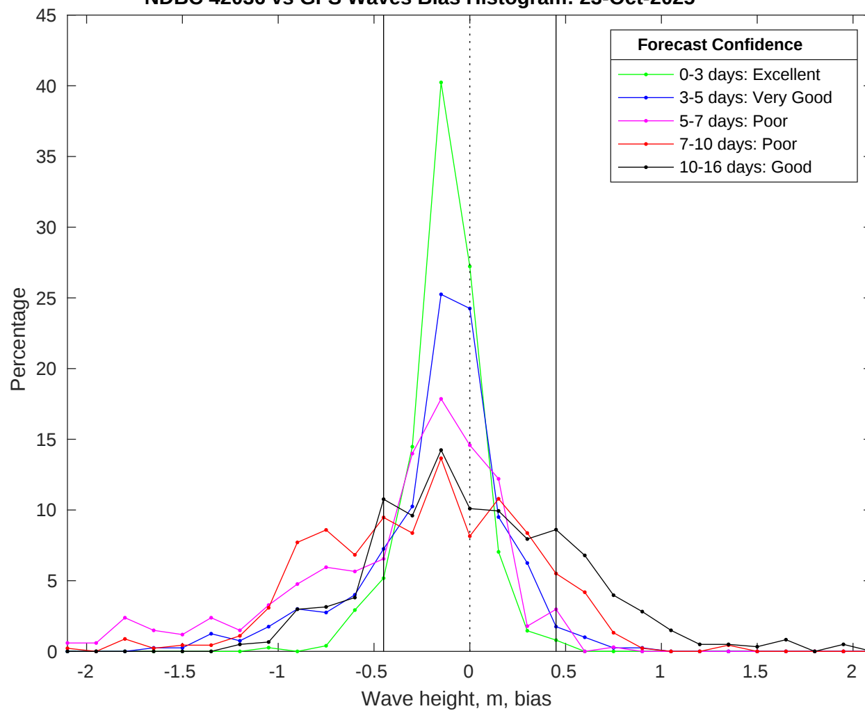
NDBC 42036 vs GFS Waves Bias Histogram: 23-Oct-2025
