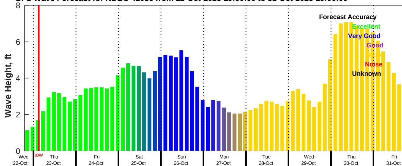
GFS Wave Forecast for NDBC 42036 from 22-Oct-2025 19:00:00 to 31-Oct-2025 19:00:00
