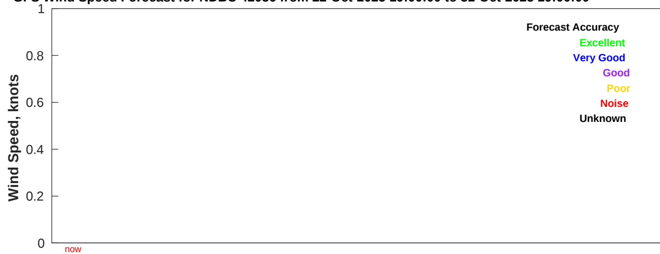
GFS Wind Speed Forecast for NDBC 42036 from 22-Oct-2025 19:00:00 to 31-Oct-2025 19:00:00
