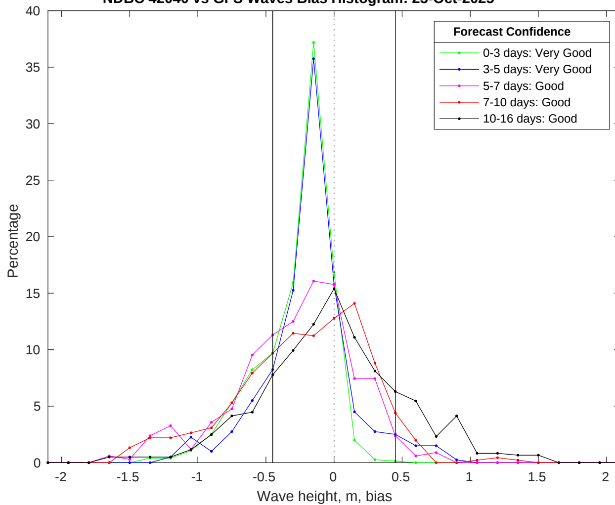
NDBC 42040 vs GFS Waves Bias Histogram: 23-Oct-2025
