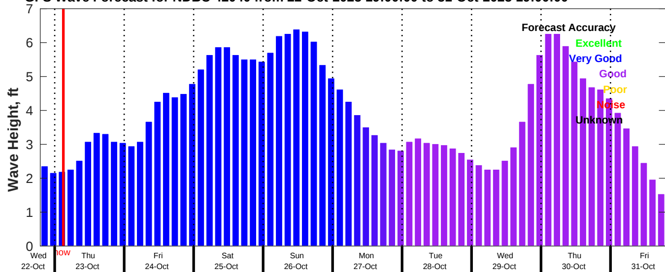
GFS Wave Forecast for NDBC 42040 from 22-Oct-2025 19:00:00 to 31-Oct-2025 19:00:00
