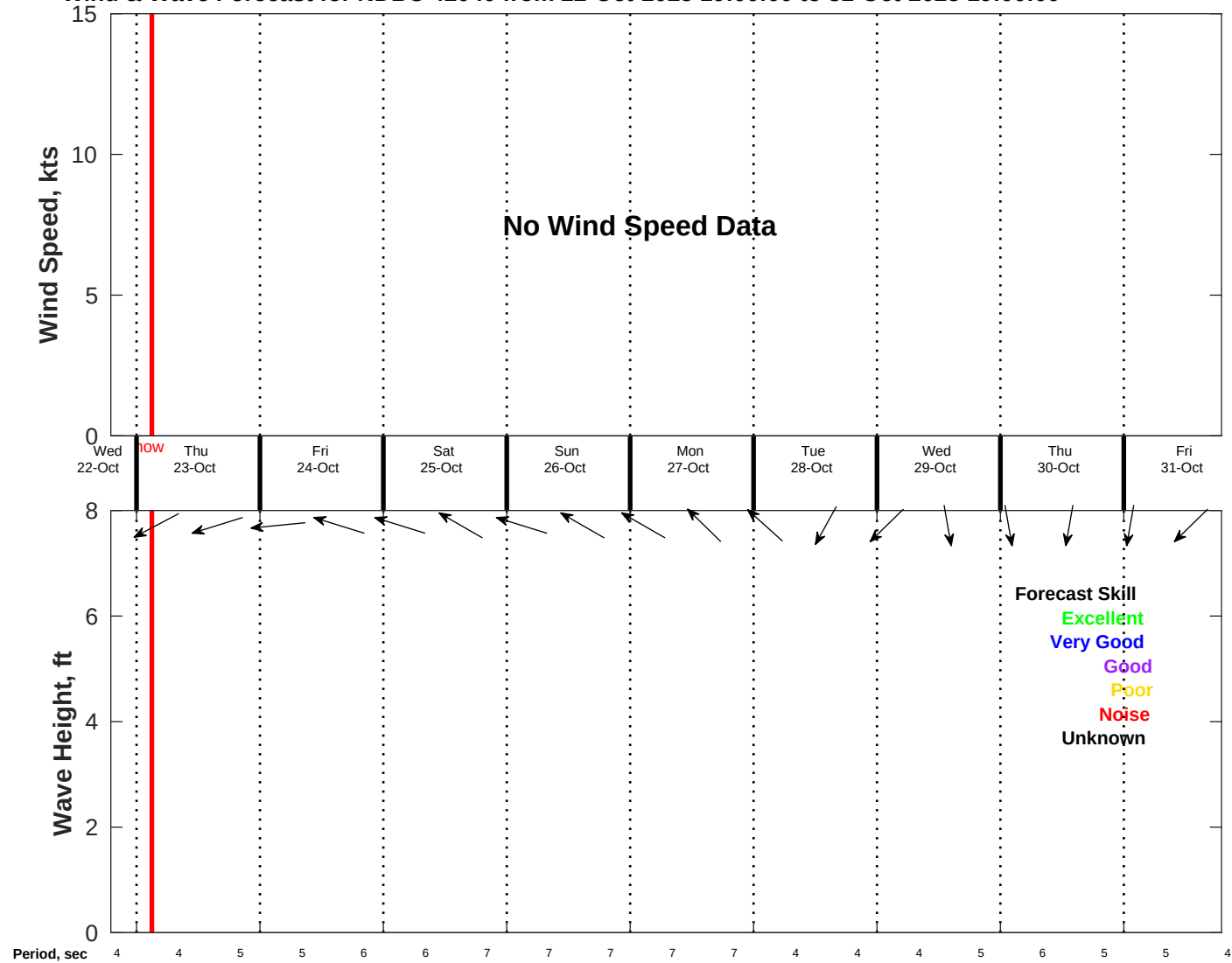
Wind & Wave Forecast for NDBC 42040 from 22-Oct-2025 19:00:00 to 31-Oct-2025 19:00:00
