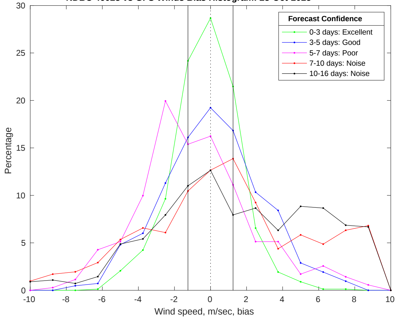
NDBC 46028 vs GFS Winds Bias Histogram: 23-Oct-2025
