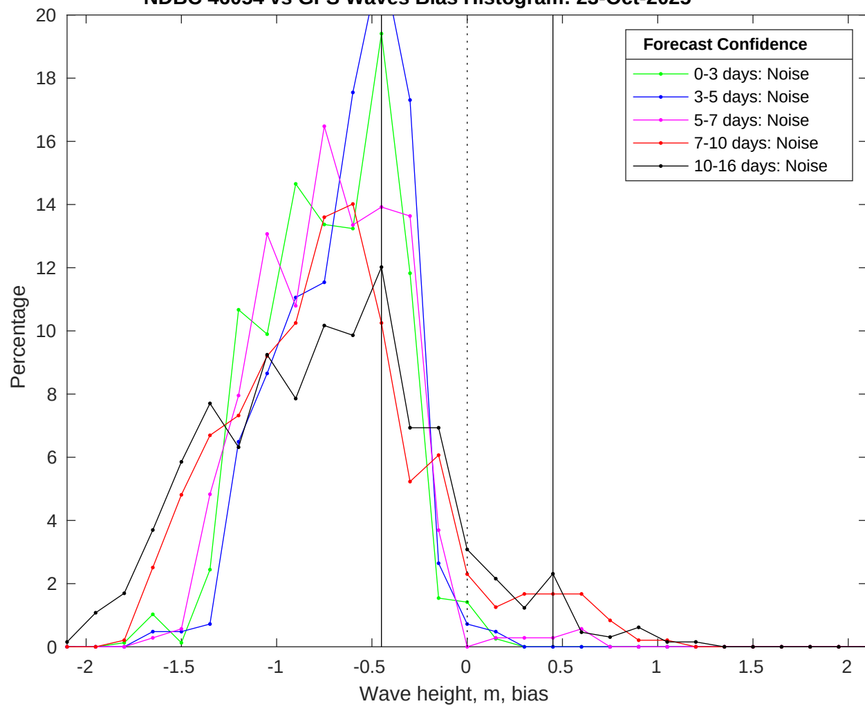
NDBC 46054 vs GFS Waves Bias Histogram: 23-Oct-2025
