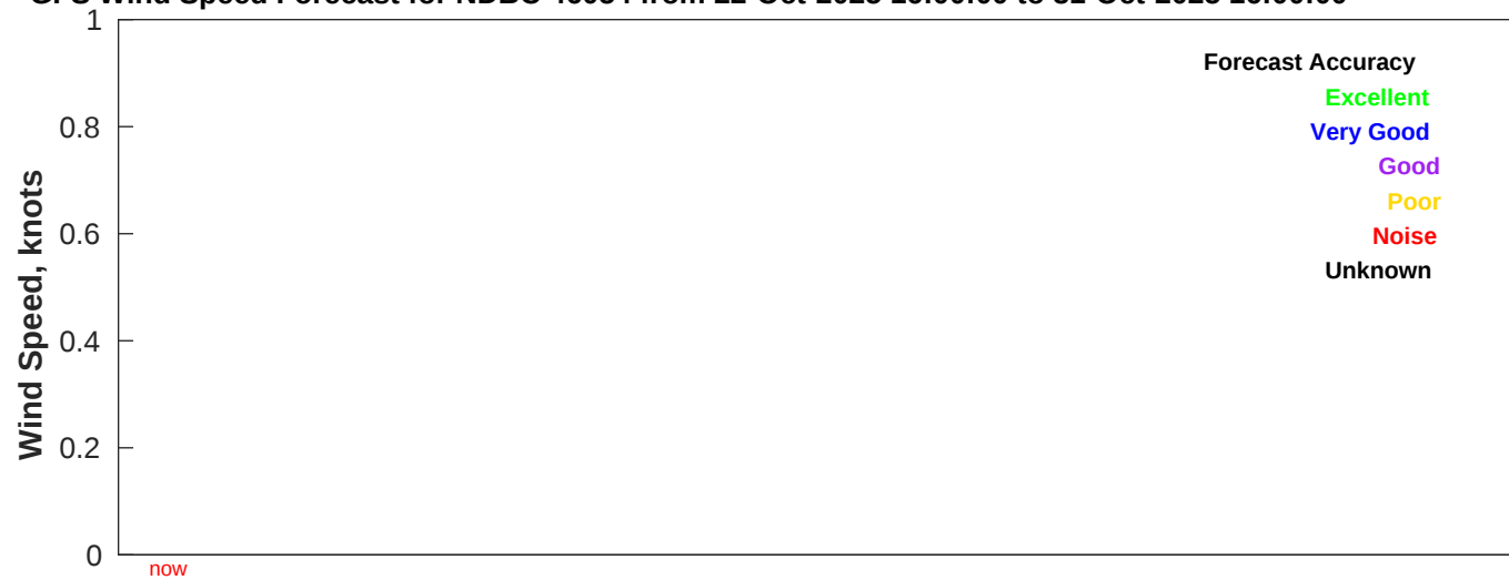
GFS Wind Speed Forecast for NDBC 46054 from 22-Oct-2025 16:00:00 to 31-Oct-2025 16:00:00
