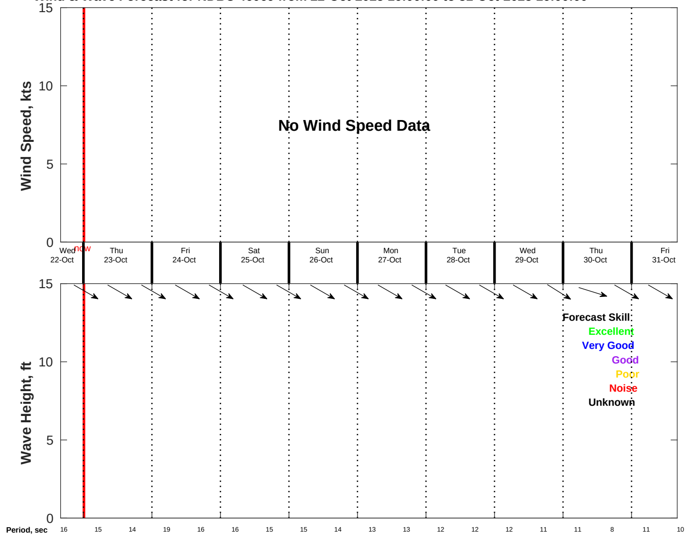
Wind & Wave Forecast for NDBC 46069 from 22-Oct-2025 16:00:00 to 31-Oct-2025 16:00:00
