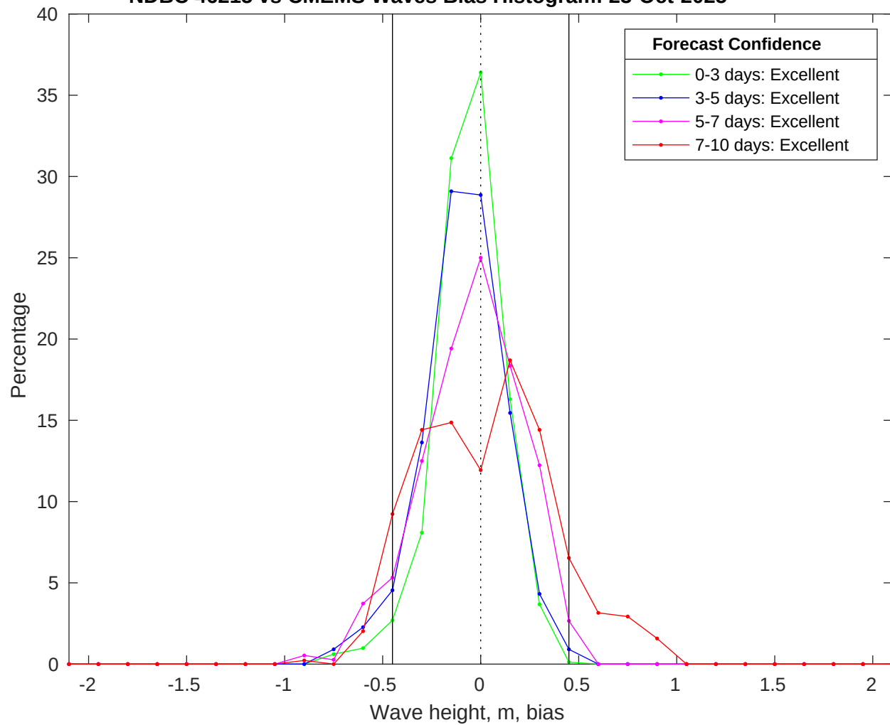
NDBC 46215 vs CMEMS Waves Bias Histogram: 23-Oct-2025
