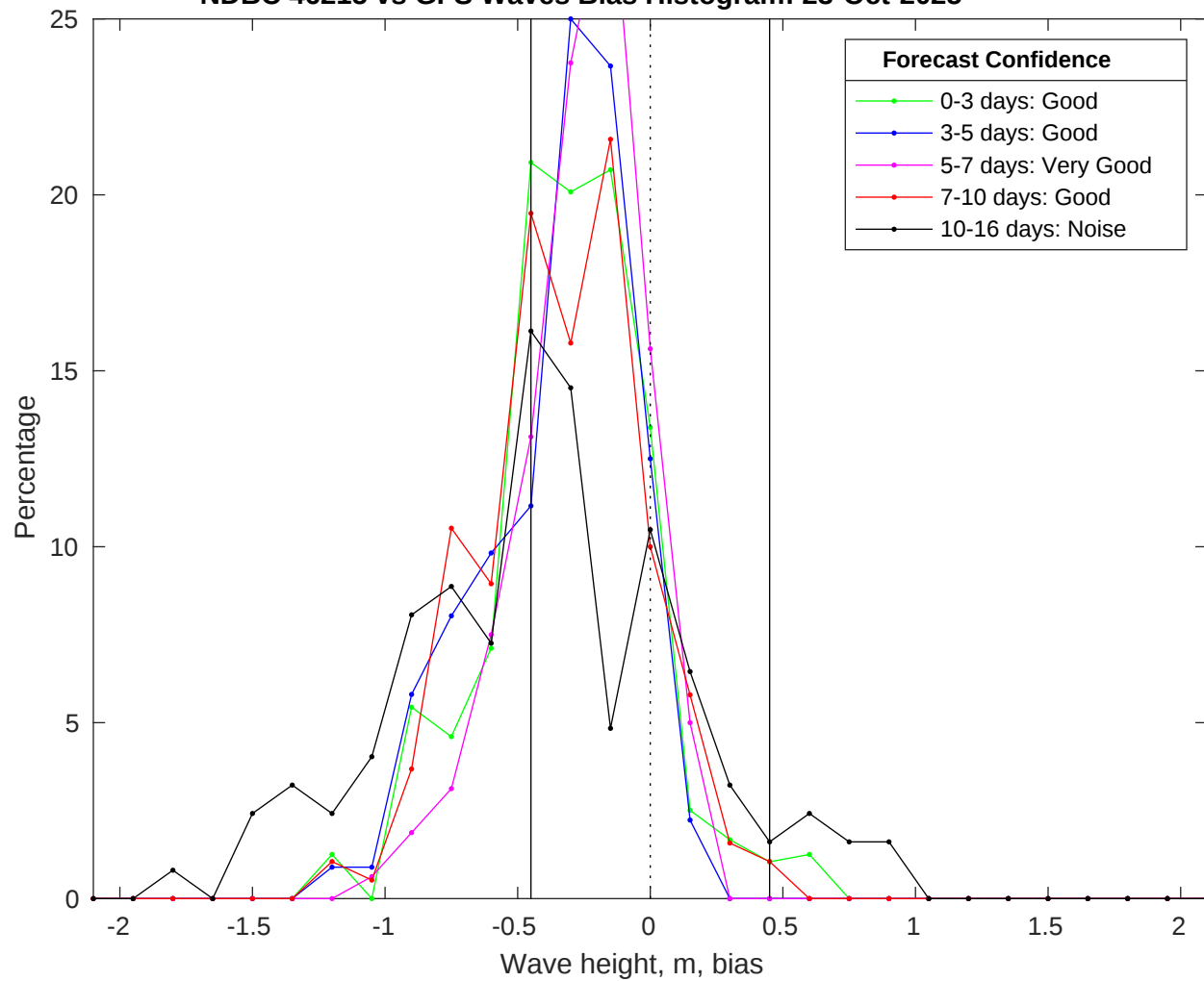
NDBC 46215 vs GFS Waves Bias Histogram: 23-Oct-2025
