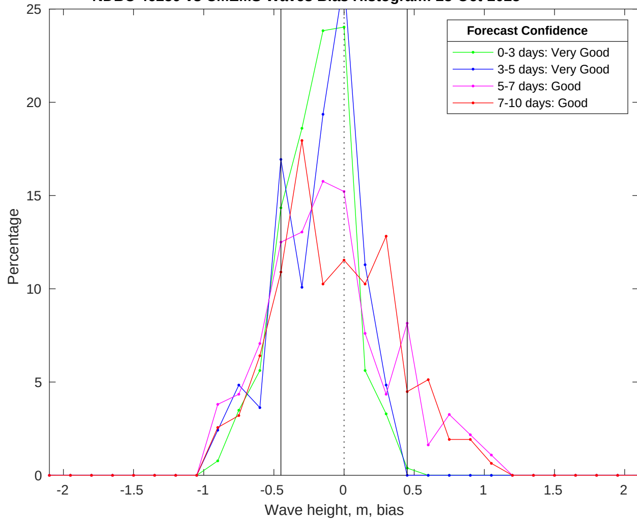
NDBC 46259 vs CMEMS Waves Bias Histogram: 23-Oct-2025
