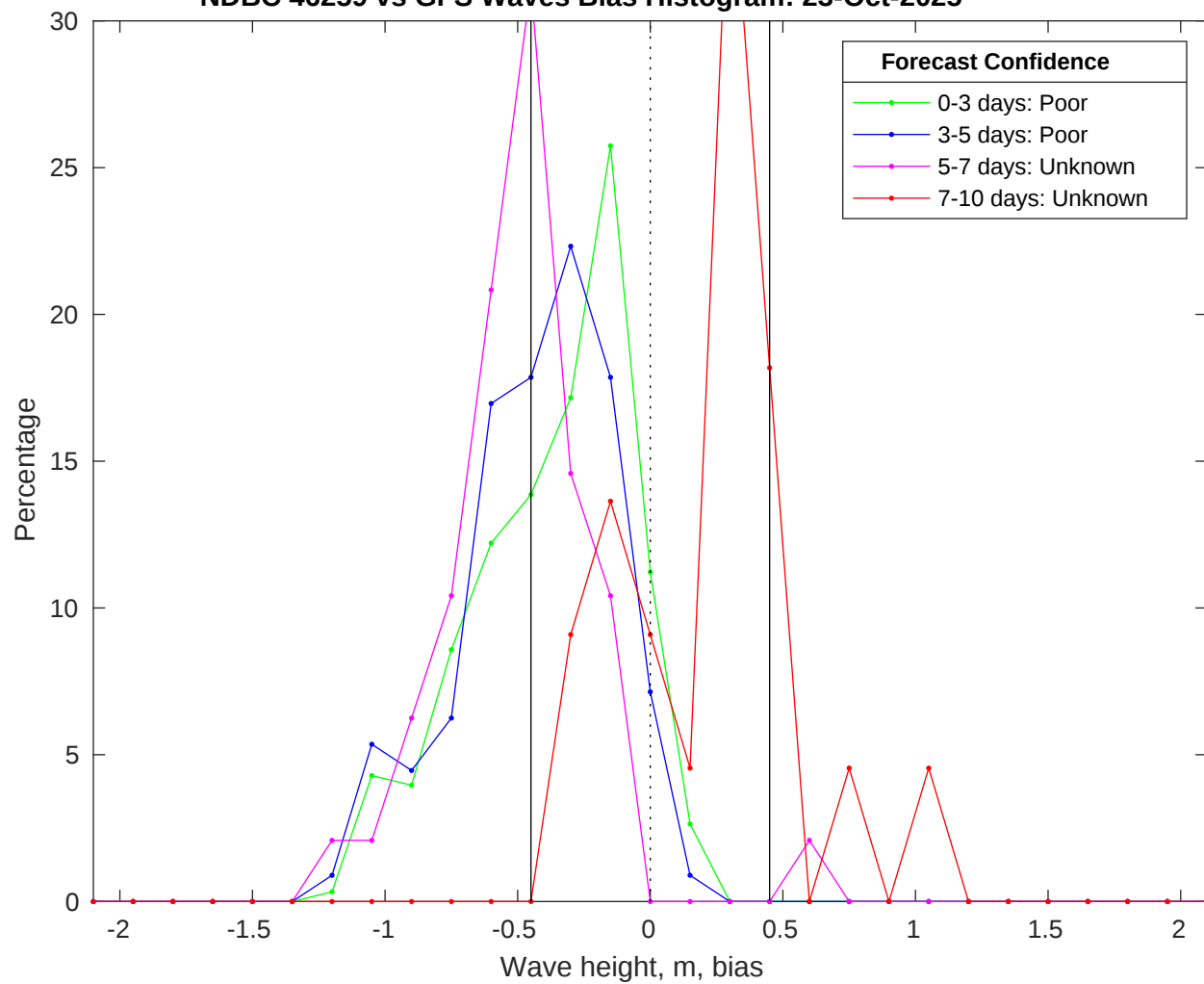
NDBC 46259 vs GFS Waves Bias Histogram: 23-Oct-2025
