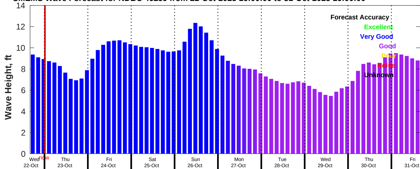
CMEMS Wave Forecast for NDBC 46259 from 22-Oct-2025 16:00:00 to 31-Oct-2025 16:00:00
